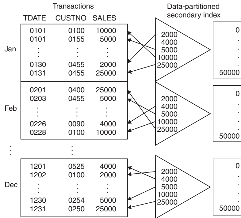
Figure 2. Example of a data-partitioned secondary index
